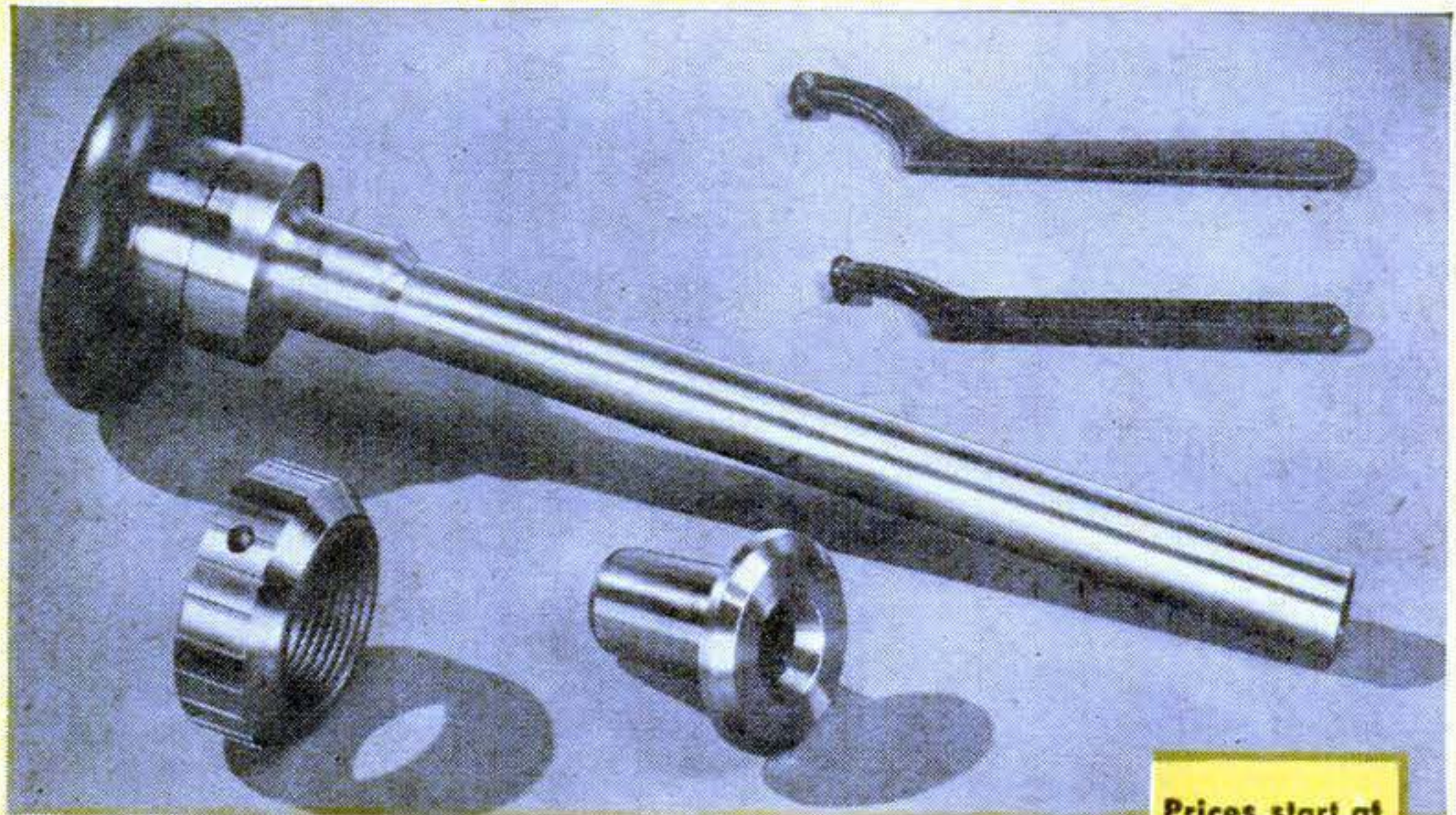
Handwheel Draw-in Collet Attachment
